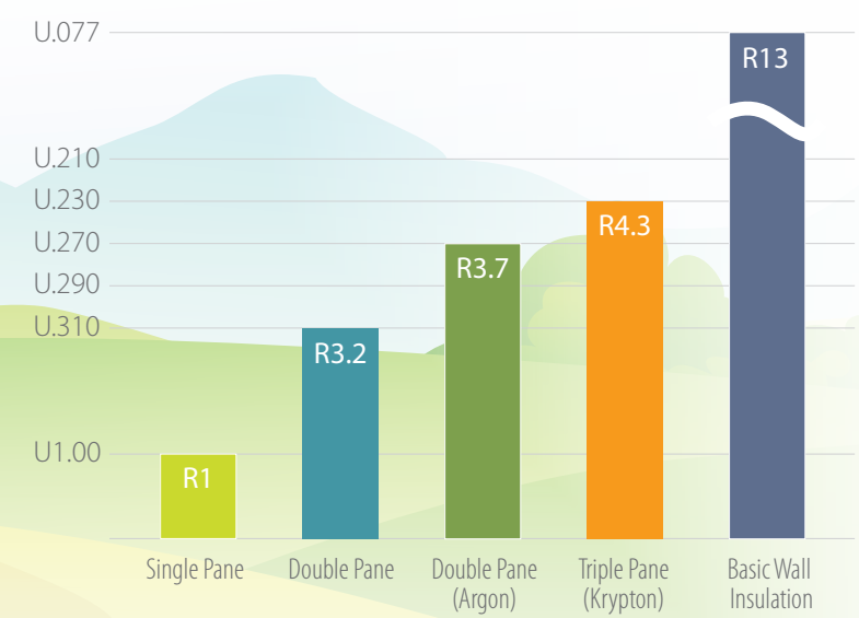
Comparative Window Example R-value vs U-value
